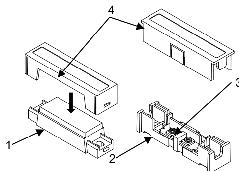
Figure 1. Magnetic contact
